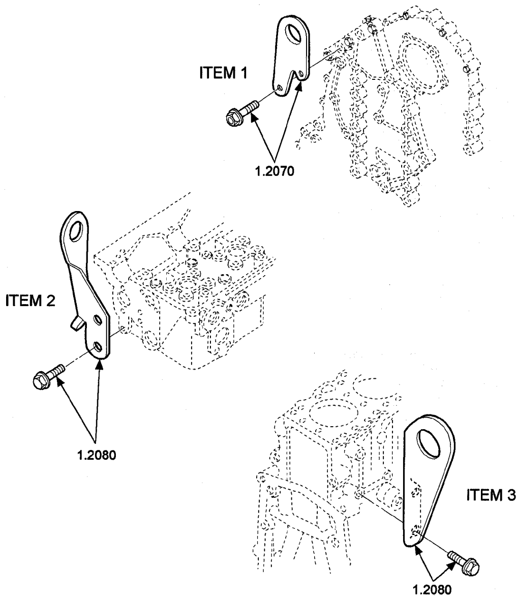
FIG. 1 ENGINE LIFTER BRACKETS
