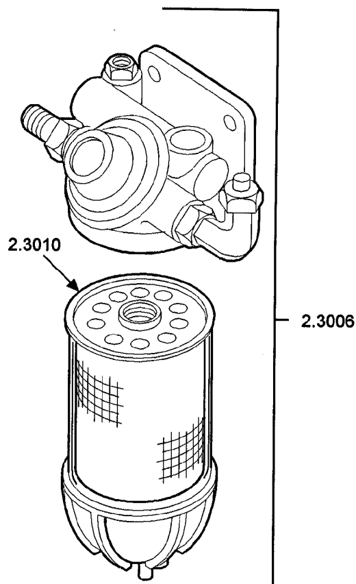
FUEL FILTER
