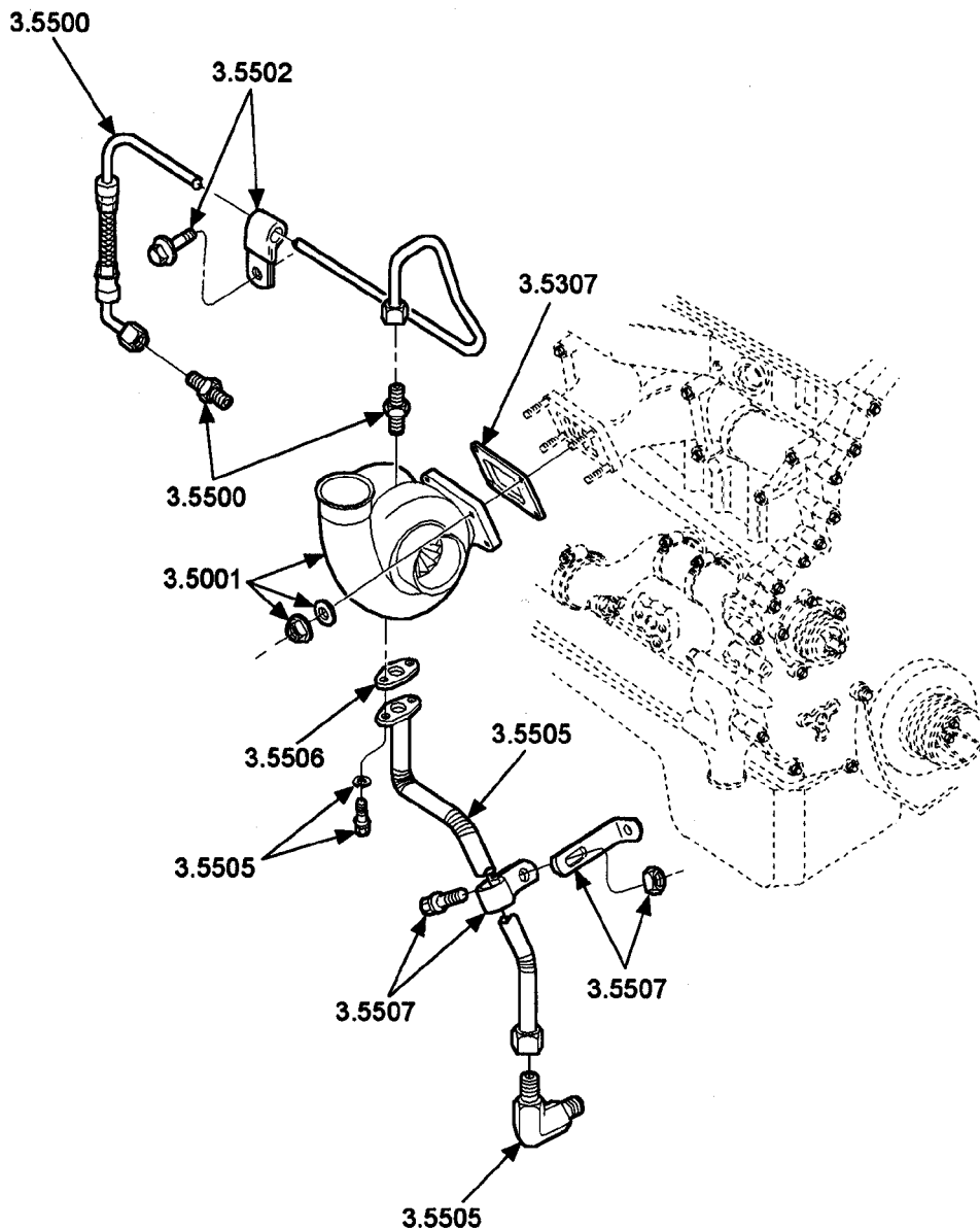
FIG.1 TURBOCHARGER INSTALLATION
