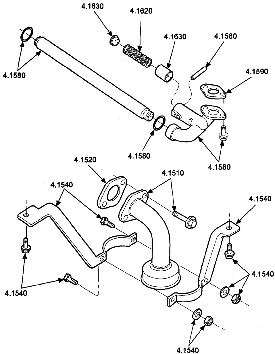
FIG. 2 OIL DISTRIBUTION SYSTEM
