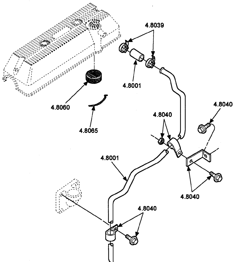
FIG. 1 BREATHER
