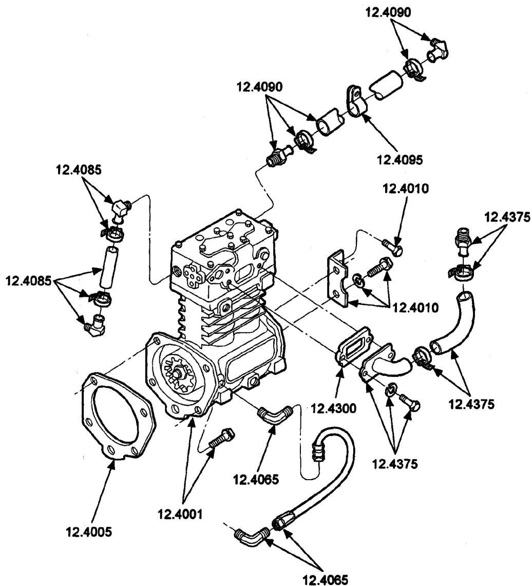
FIG. 2 AIR COMPRESSOR ASSEMBLY
