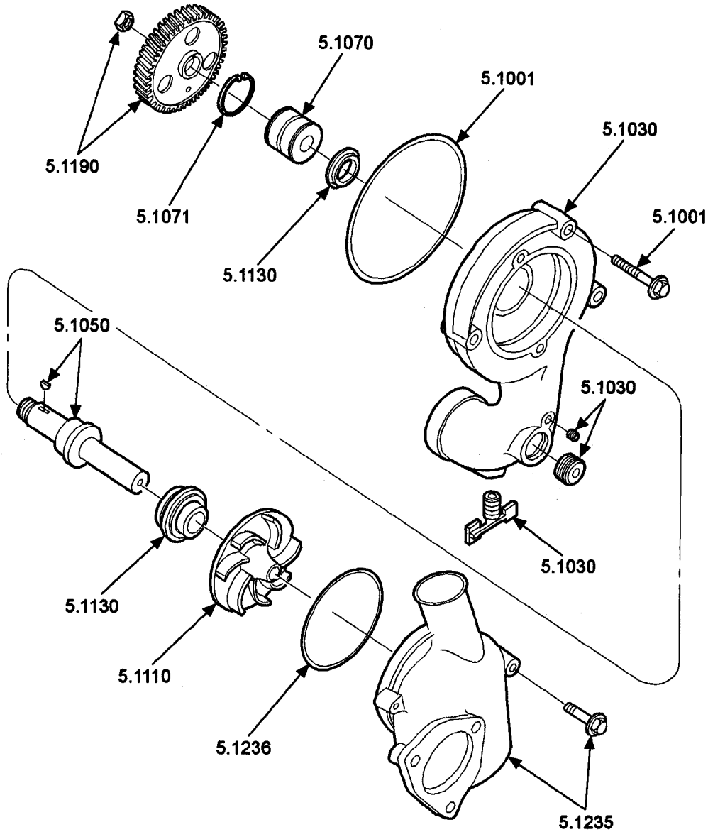
FIG. 1 WATER PUMP AND COVER ASSEMBLY
