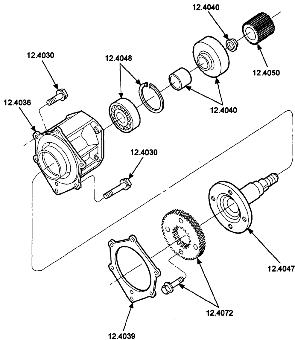
FIG. 3 AIR COMPRESSOR DRIVE ASSEMBLY
