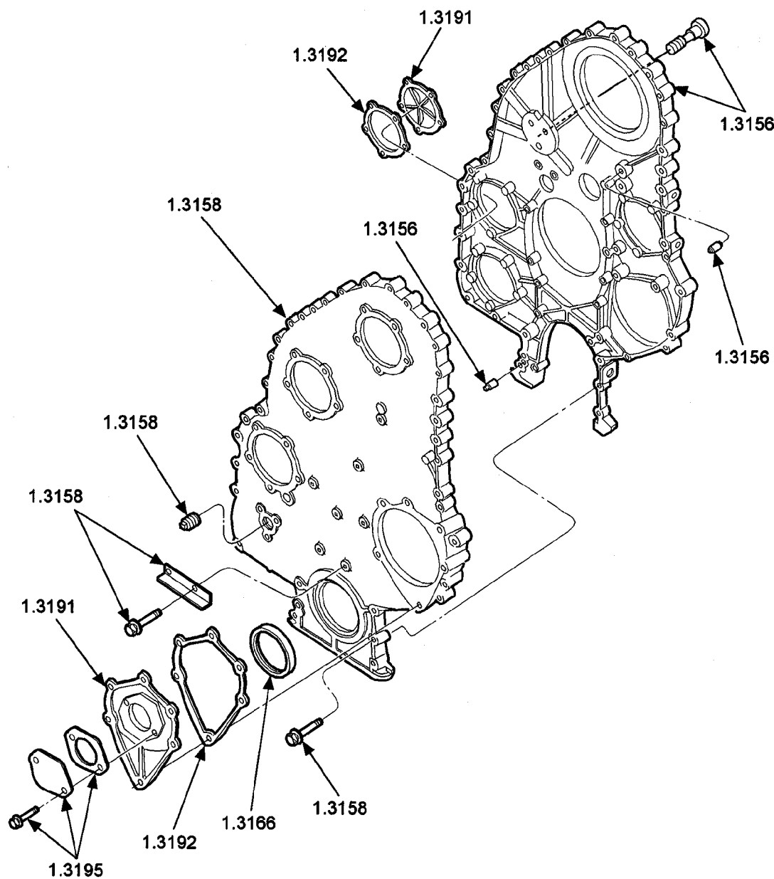
FIG. 1 GEAR CASE AND FRONT COVER ASSEMBLY
