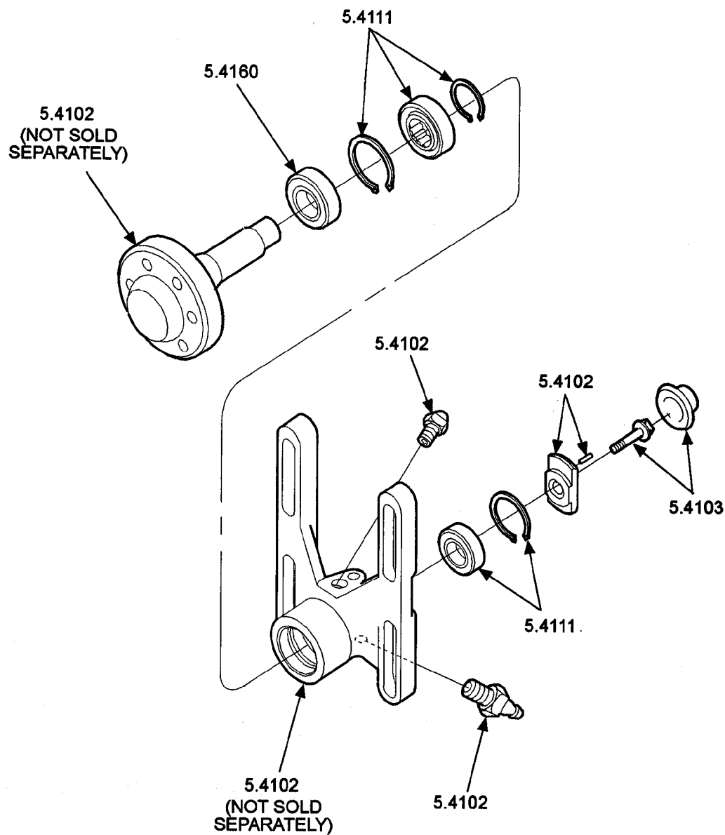
FIG. 2 SPINDLE AND HOUSING ASSEMBLY
