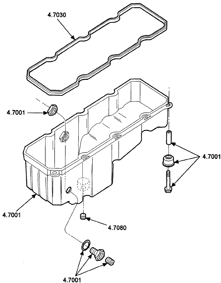
FIG. 1 OIL PAN ASSEMBLY
