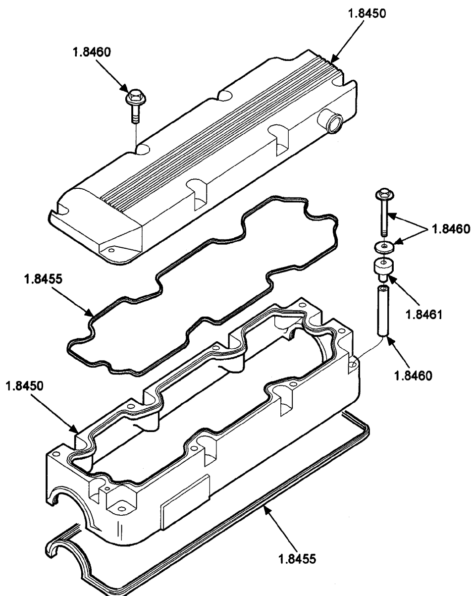
FIG. 2 ROCKER COVER
