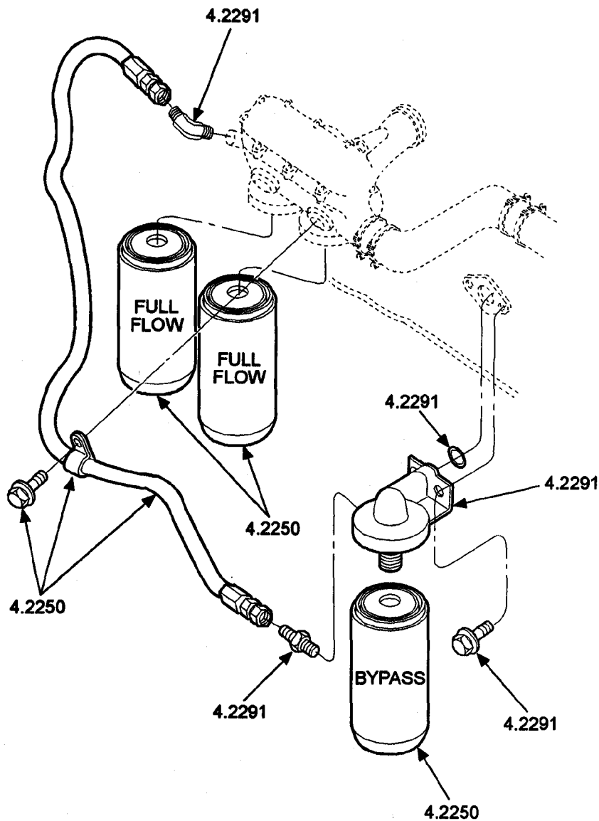
FIG. 2 OIL FILTERS
